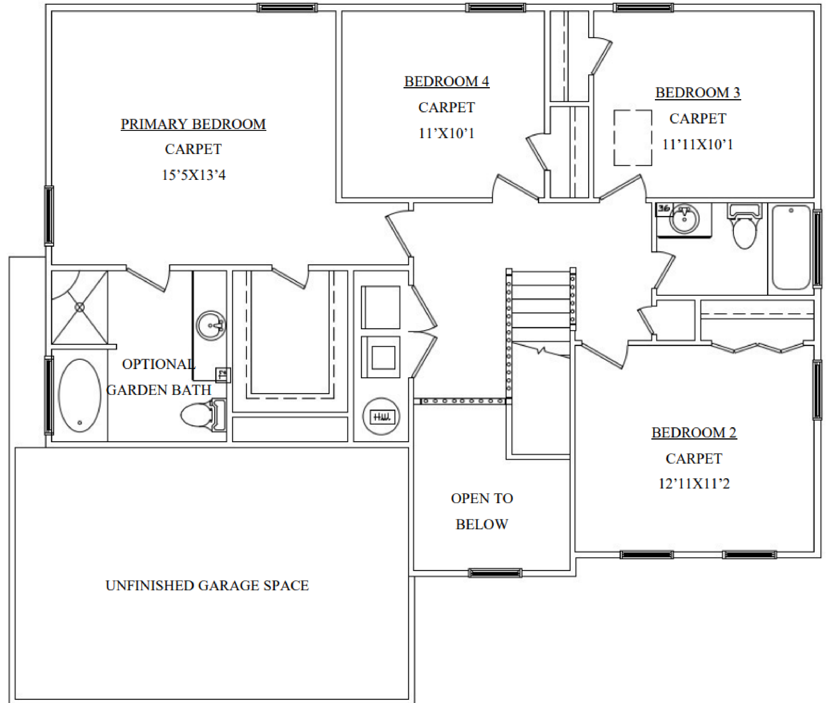
OPTIONAL 2ND FLOOR LAYOUT
