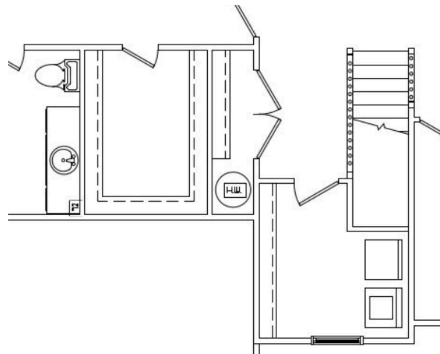
OPTIONAL 2ND FLOOR LAYOUT
